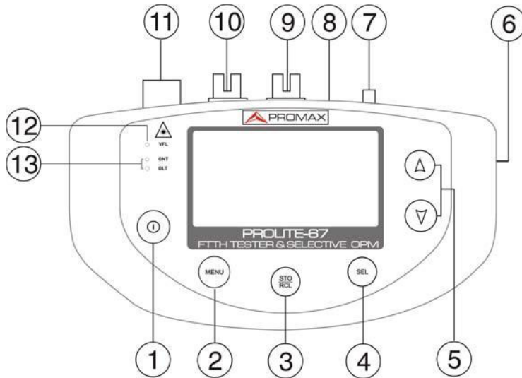
Figure 2.- Front View.
