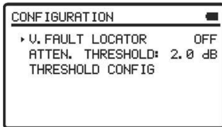
Figure 5.- CONFIGURATION screen.
