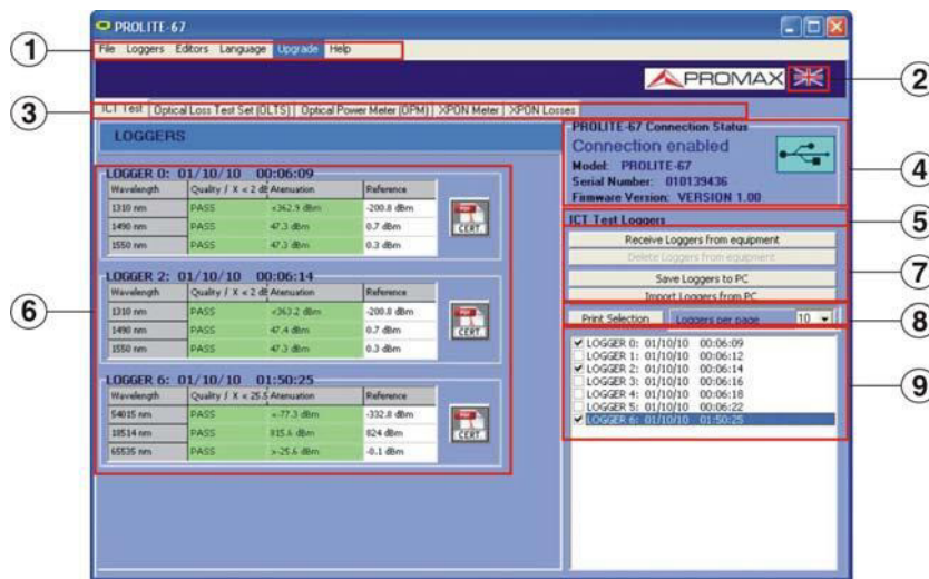
Figure 25.- Main window.
